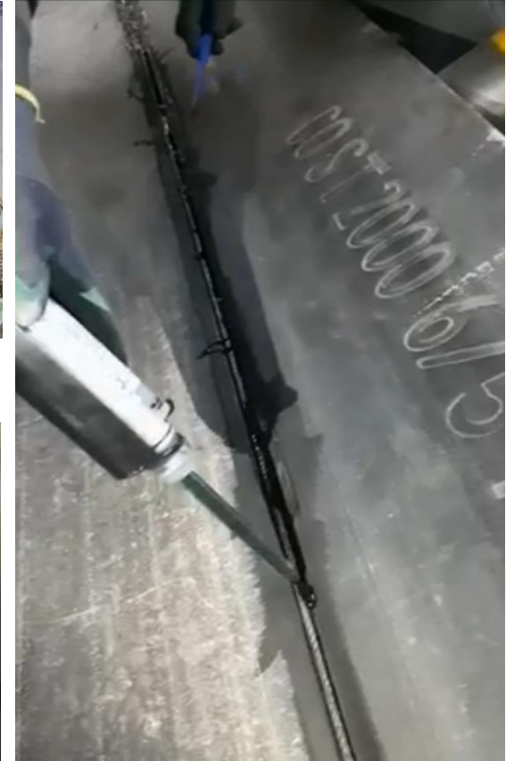
Steel cord belt long rip repair
