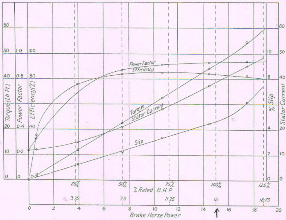
FIG. 1.16. DIRECT DETERMINATION OF THE CHARACTERISTIC OF A THREE-PHASE INDUCTION MOTOR
