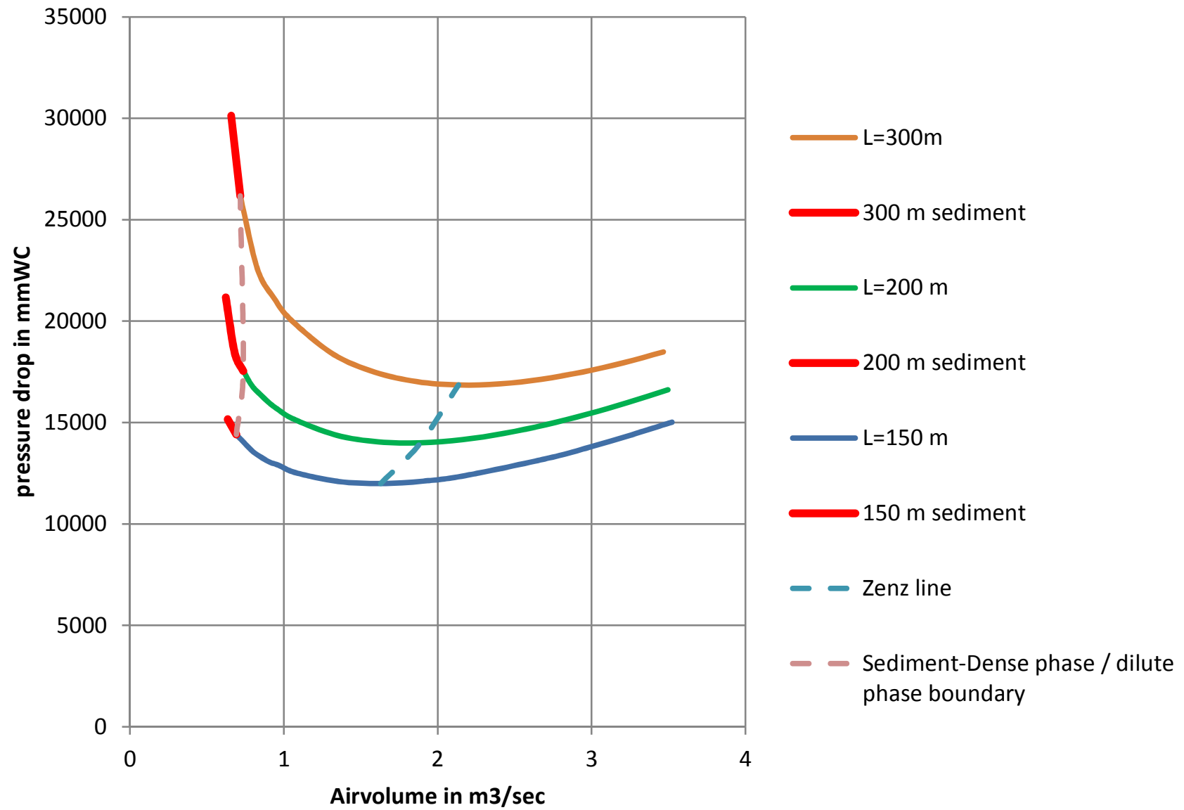
Zenz diagram Cement -150 t/hr - 254/304mm (Yarca.nl)
