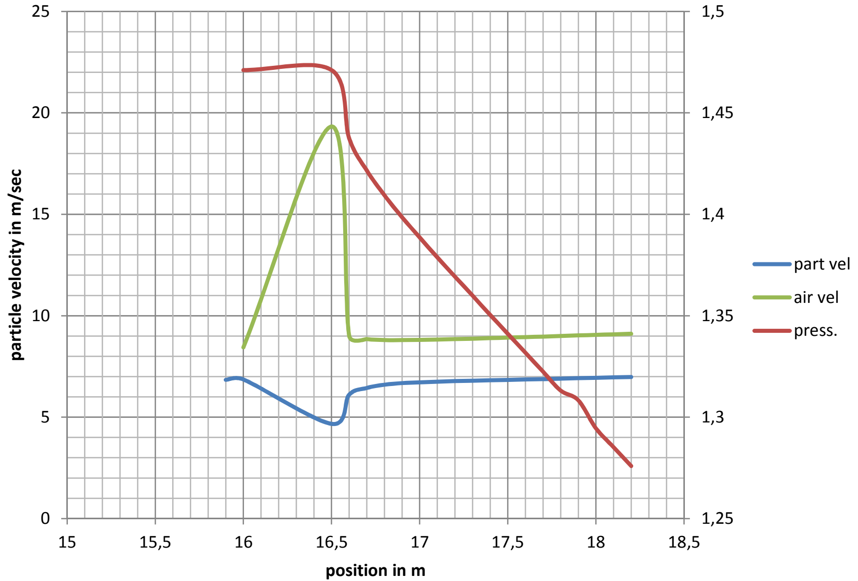
horizontal to vertical bend (Cement - pipe 200 mm)
