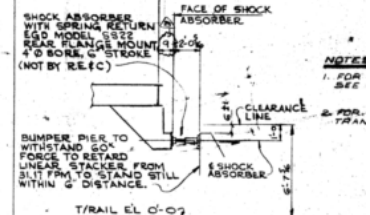
SECTION A (AS SHOWN - SOUTH SIDE) (OPP. HAND - NORTH SIDE)
