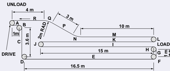
Fig. 24 Sideview of conveyor circuit
