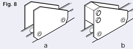
(a) S attachment outer plate; assembled on one or both sides of chain as required. (b) Pusher attachment.
