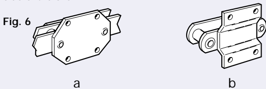
(a) G2 attachment outer plate. (b) G2 attachment, welded or rivetted to link plate.
