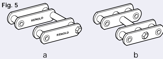
(a) Staybar bolted through hollow bearing pin. (b) Staybar assembled through outer or inner link.
