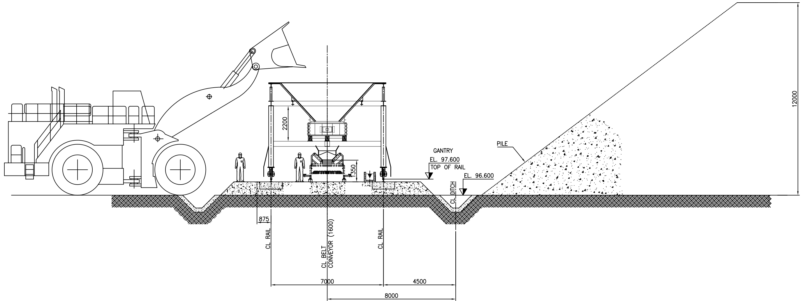
ELEVATION OF EMERGENCY HOPPER
