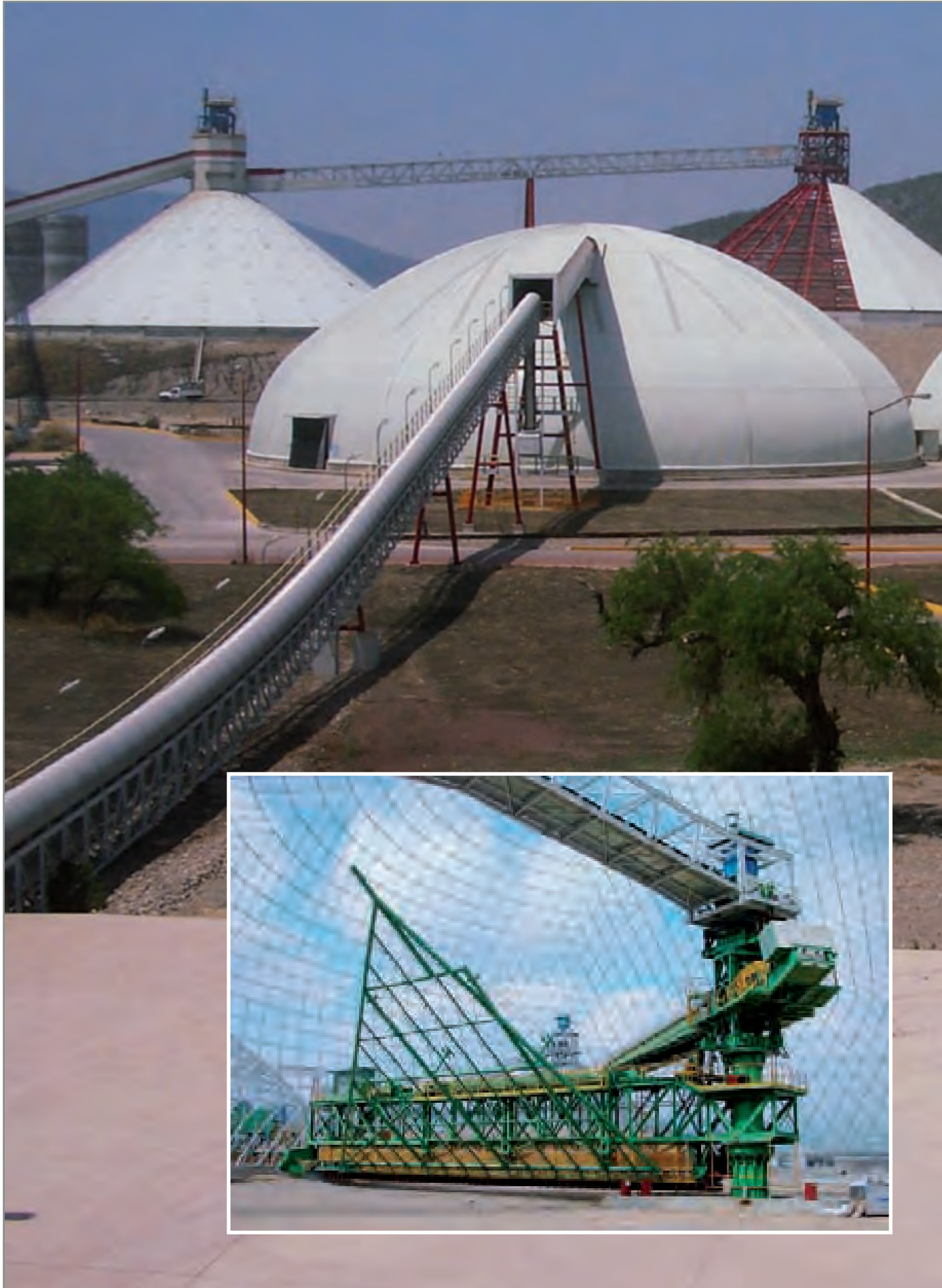
Pre-blending systems: different types of stackers and reclaimers; circular, lateral and frontal.
