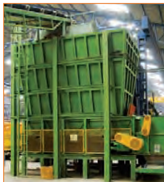
Different types of metal apron feeders. Special versions with additional hopper, capacity up to 300 cubic meters and over, are also available.
