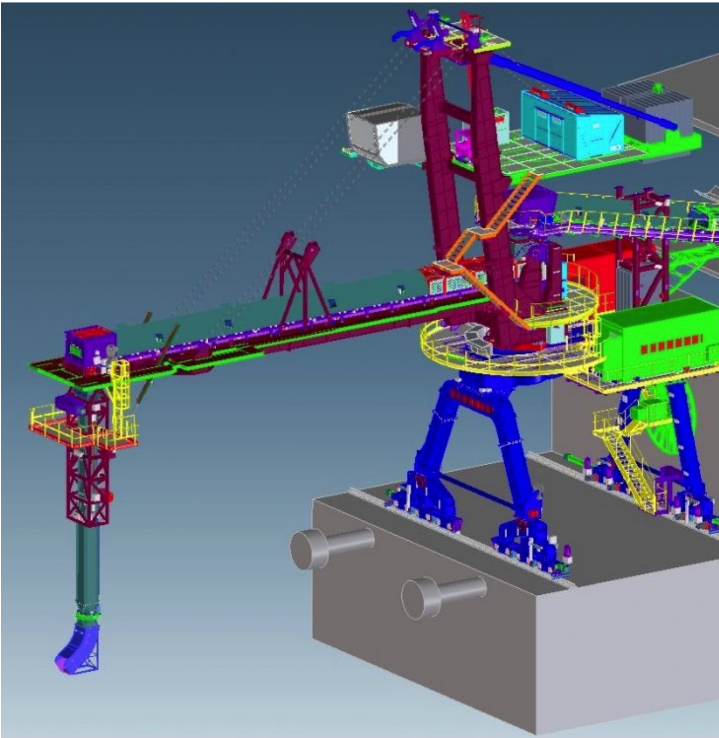
3D drawing of the shiploader in the design phase. (Picture: ©Bedeschi S.p.A.)
