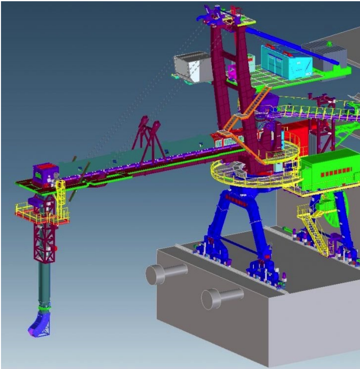
3D drawing of the shiploader in the design phase. (Picture: ©Bedeschi S.p.A.)
