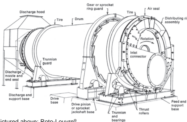
Pictured above: Roto-Louvre®
