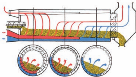
Pictured above: Dryer / Cooler
