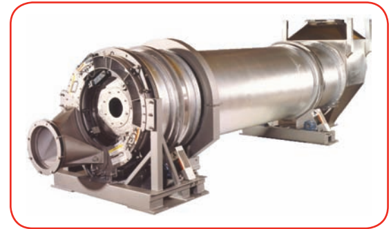
Pictured above: Roto-Louvre®
